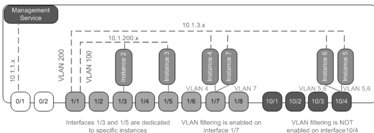
Figure 1. Network topology of an SDX appliance with Management Service and Citrix ADC instances distributed across networks
