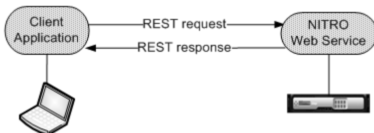
Figure 1. NITRO workflow
